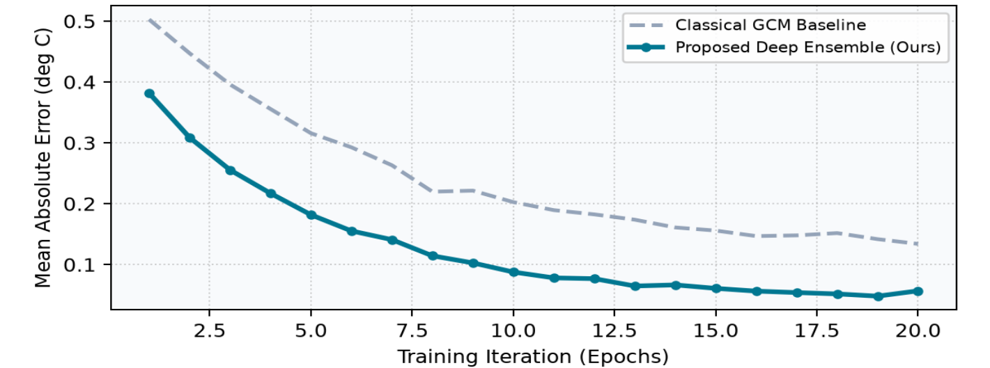
Figure 1: Global Atmospheric Temperature Prediction Convergence
